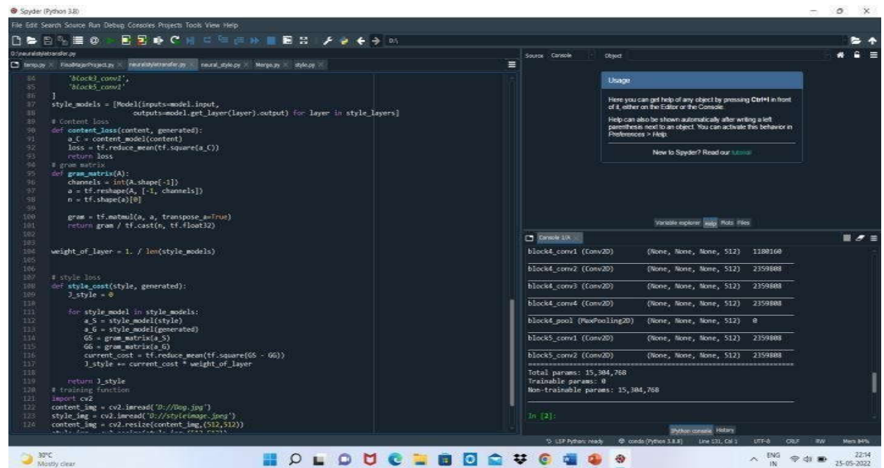
Figure 4.1-4.3-Code Execution
