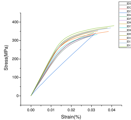
Fig.5: Stress-strain comparison plot
