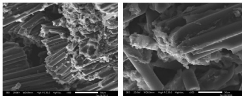
Fig. 11: SEM of impact fractured specimen surface
