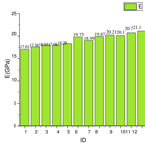
Fig.6: Young's modulus comparison plot
