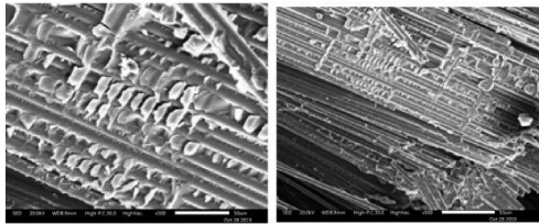
Fig. 10: SEM of the tensile fractured specimen surface
